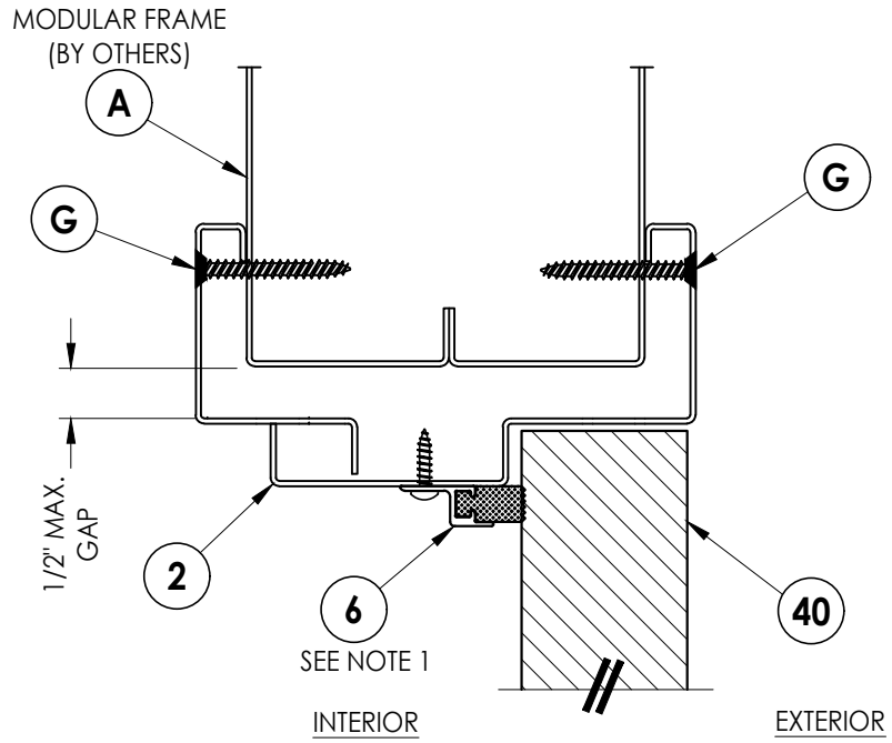
1 VERTICAL CROSS SECTION 4 Modular Frame Installation
